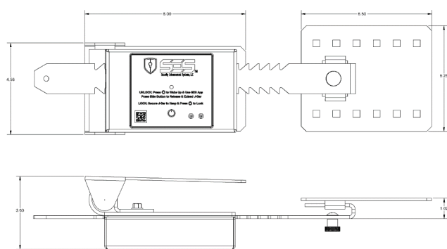
SWING MOUNT
