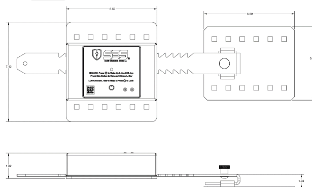
RIGID MOUNT
